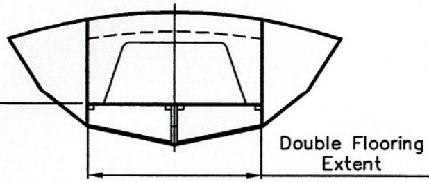
BULKHEAD No.2
